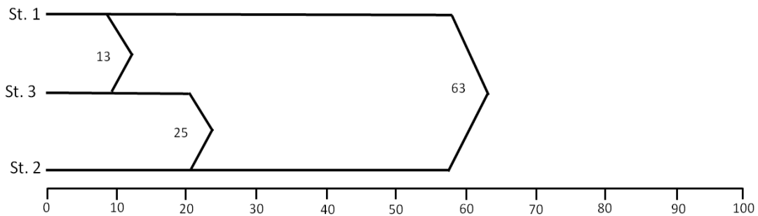
Fig. 12: Dendrograph based on Jaccard's similarity index of Cladocera at the three stations of Shatt Al-Arab River between January and November 2013 on a seasonally basis.
