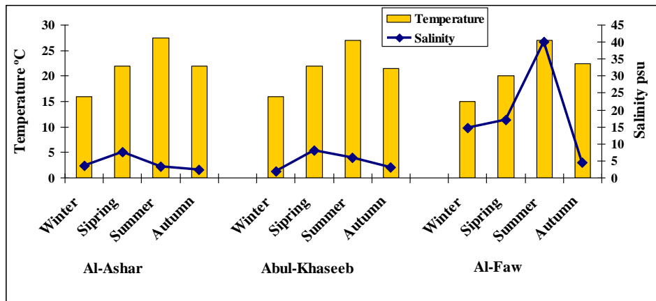
Fig. 2: Water temperatures and Salinity at three stations during the study period.
