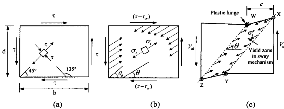
Figure (1): Phase in girder behavior up to collapse (a) Unbuckling behavior (b) Post-buckling behavior (c) Collapse behavior.
