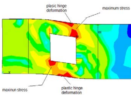
g) Beam BS3
