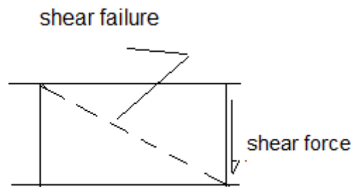
Figure (7): Failure for solid and small web opening ( d_o=50 mm) girders
