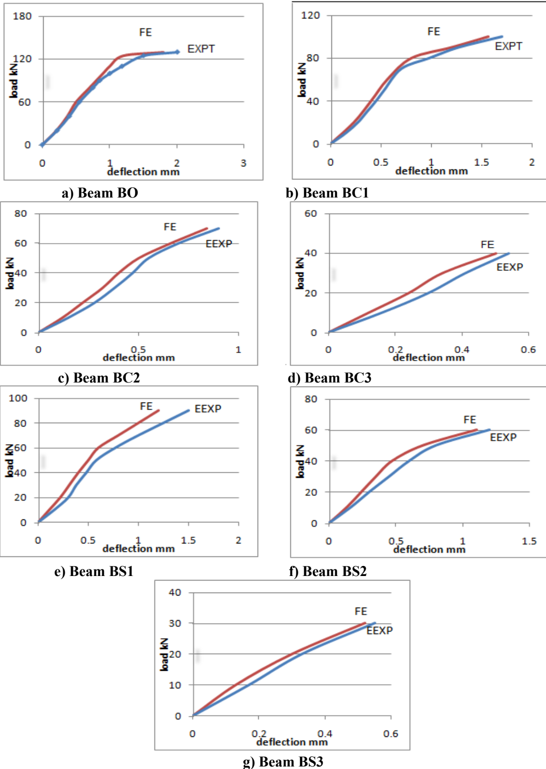
Figure (6): Variation of deflection with load for all beams.
