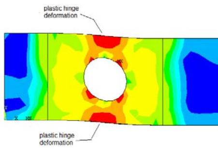
d) Beam BC3
