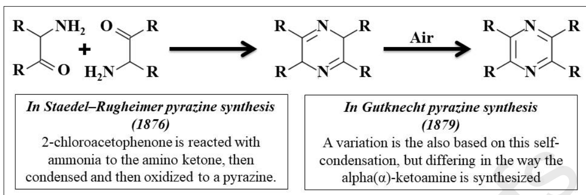
Figure-5: Pyrazine synthesis by condensation reaction.
