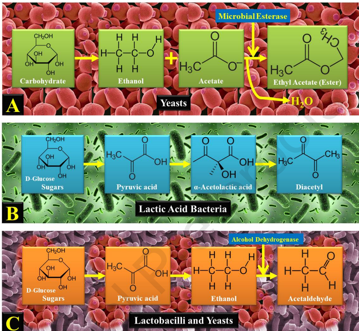
Figure-4: Synthesis of different microbial VOCs. (A) Ester (ethyl acetate) synthesis from carbohydrate through yeasts, (B) Diacetyl synthesis from carbohydrate in LAB, (C) Acetaldehyde synthesis from carbohydrate in lactobacilli and yeasts.
