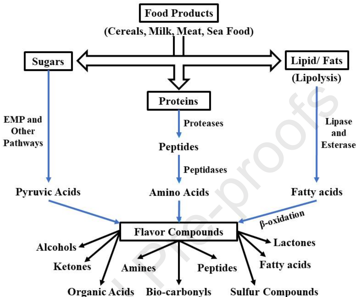
Figure-3: Biosynthesis of flavours by different microorganism in various food products.
