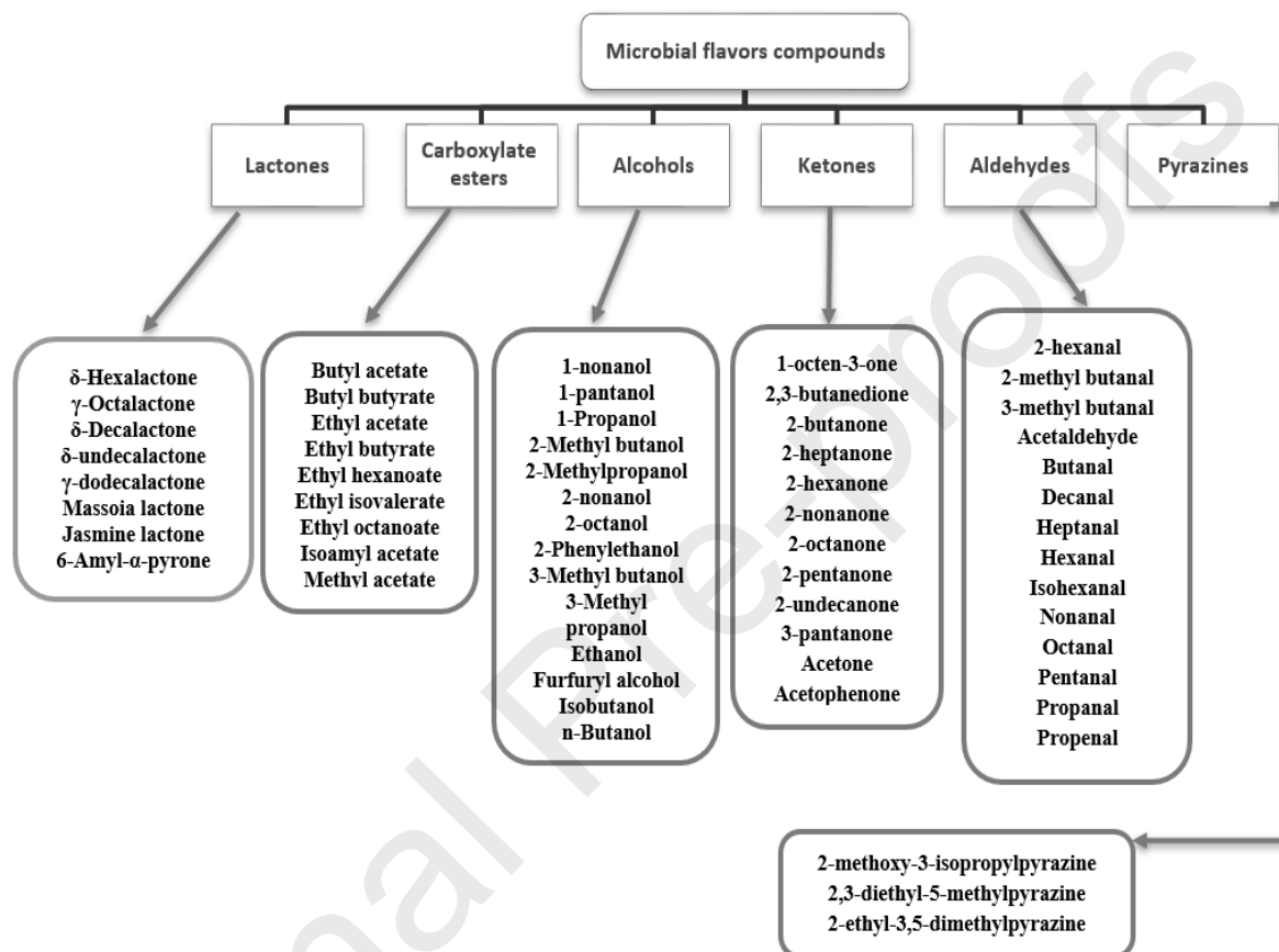
Figure-2: Classification on the basis of chemical compositions for microbial VFCs.
