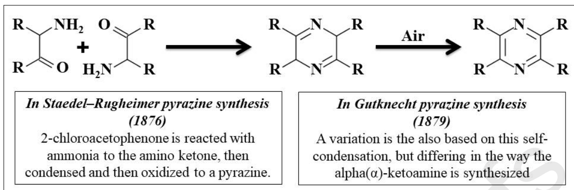
Figure-5: Pyrazine synthesis by condensation reaction.
