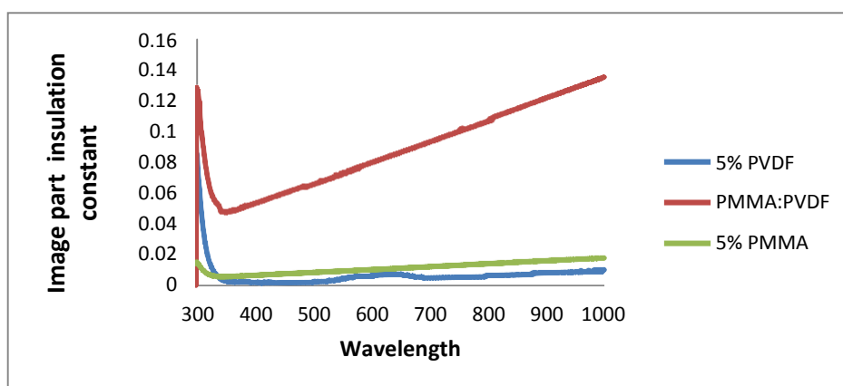
Fig(7) : Relationship between the image part of dielectric constant and the wavelength
