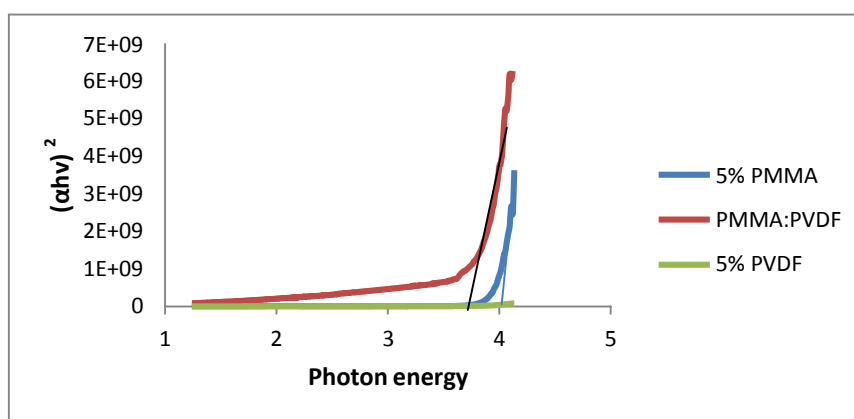
Fig (8): Relationship between (\alpha h\nu)^2 and photon energy
