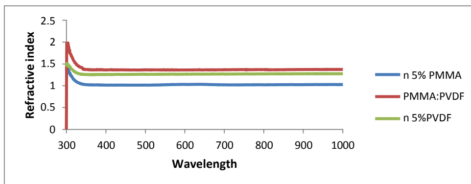
Figure (4): Relationship between the refractive index and the wavelength
