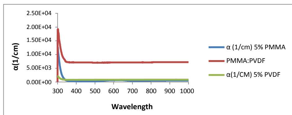
Fig(3): Relationship between absorption coefficient and wavelength
