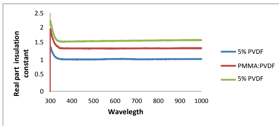
Fig(6): Relationship between the real part of dielectric constant and the wavelength
