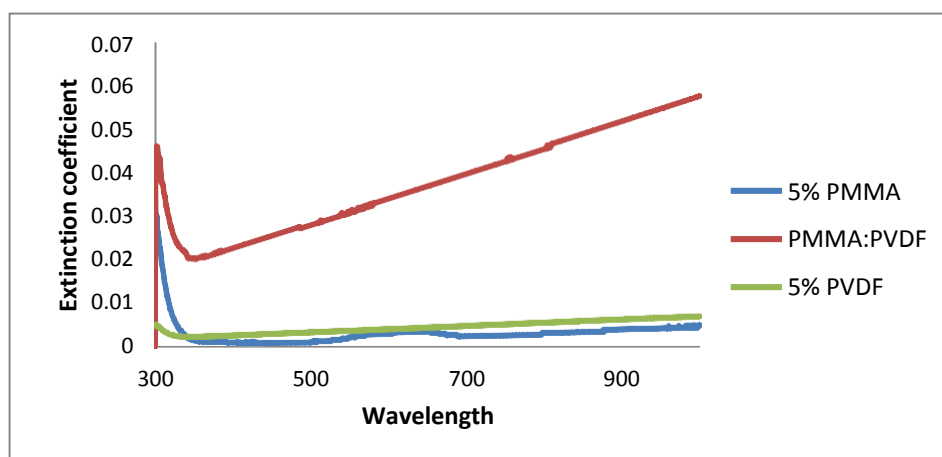
Fig (5): Relationship between Extinction coefficient and the wavelength
