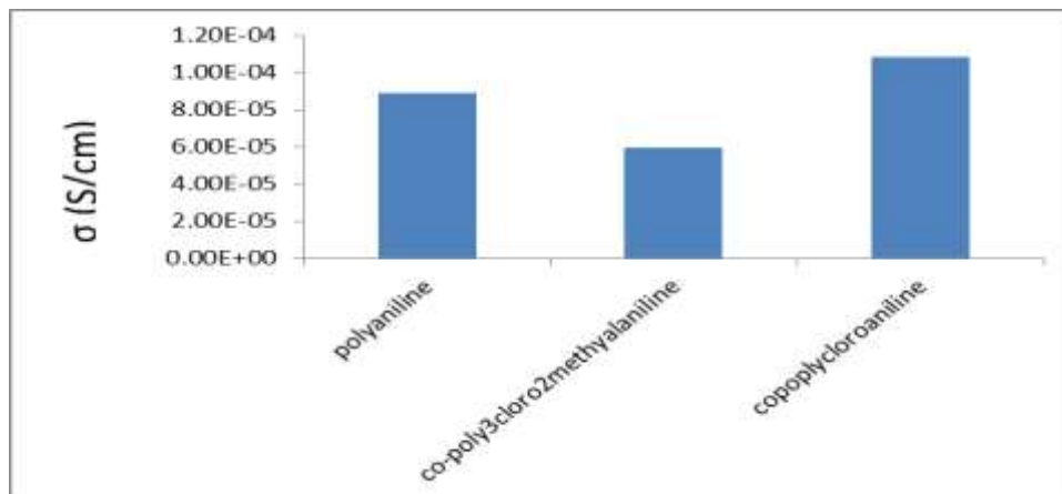
Fig(7) shows the conductivity for (poly Aniline, co-poly(3cloro-2methelaniline,co-poly(2-cloroaniline))),deposited on glass substrate clear from the figure that increasing conductivity for co-poly(cloroanile) this behavior same the behavior in figure (5)
