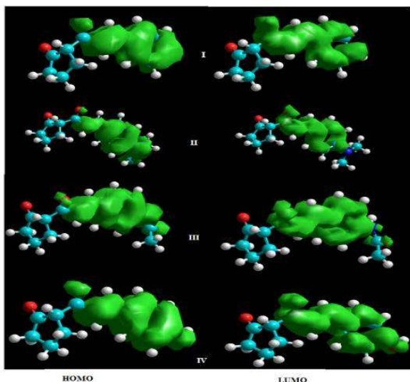
Figure 7: Highest occupied molecular orbital (HOMO) and lowest unoccupied molecular orbital (LUMO) of compounds I – IV
