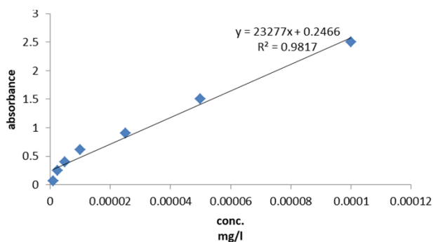
Figure 10: Absorbance of complex 3 spectra versus conc
