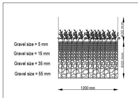
Fig. 4 Cross-section of (HSFS CWs) media.
