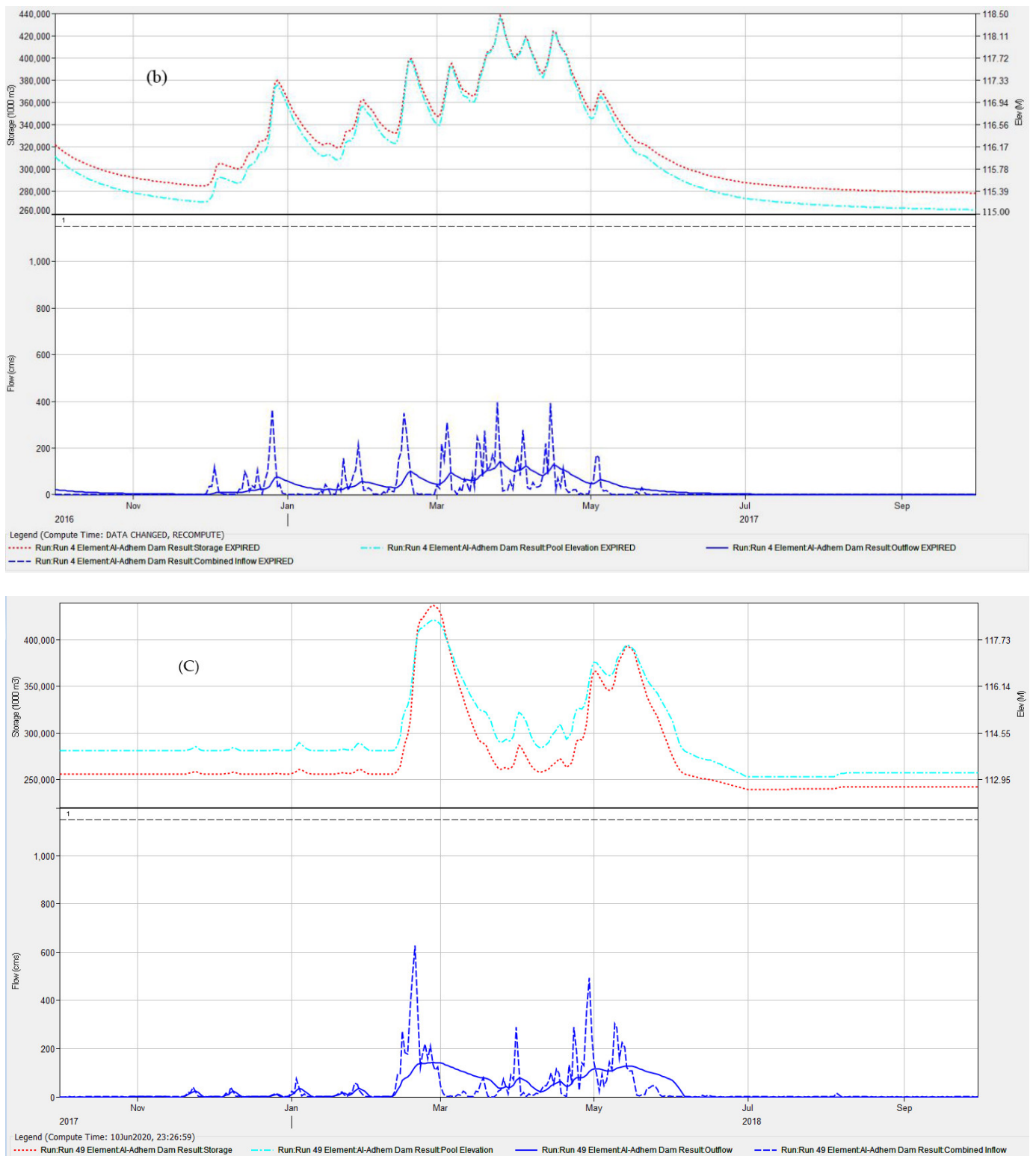
Figure 12. The simulation run for the AI-Adhaim reservoir concerning the intervals (a) 2015–2016; (b) 2016–2017; and (c) 2017–2018.
