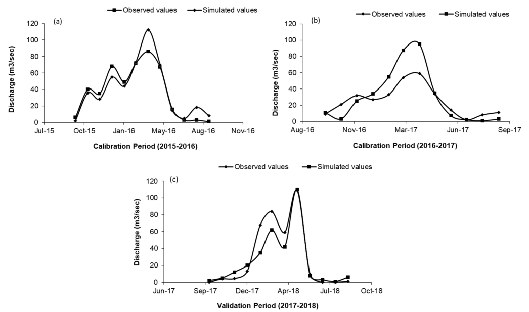
Figure 9. Observed and simulated discharge values for the dam outlet (a) calibration of 2015–2016; (b) calibration of 2016–2017; and (c) validation of 2017–2018.
