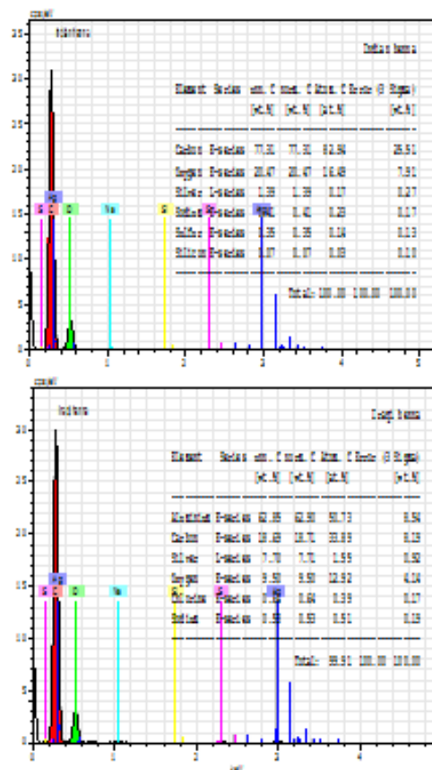
Figure 4: EDS analysis of prepared silver nanoparticles from Indian and Iraqi henna
