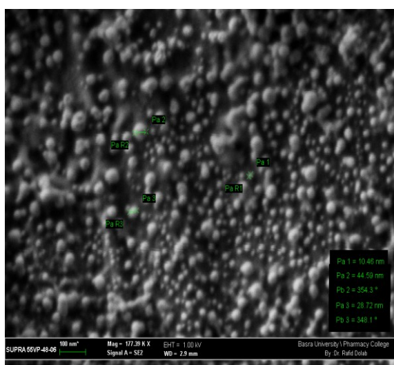
Figure 3: Demonstrations the shape and size of silver nanoparticles prepared by using Indian and Iraqi henna.
