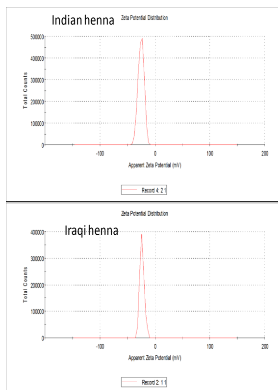
Figure 6: shows the zeta potential of silver nanoparticles prepared by different types of henna.
