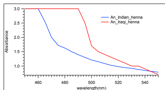
Figure 2: UV-visible absorption spectra of silver nanoparticles, which prepared from Indian and Iraqi henna
