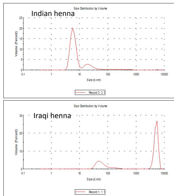
Figure 5: shows the size distribution of silver nanoparticles prepared by different types of henna.
