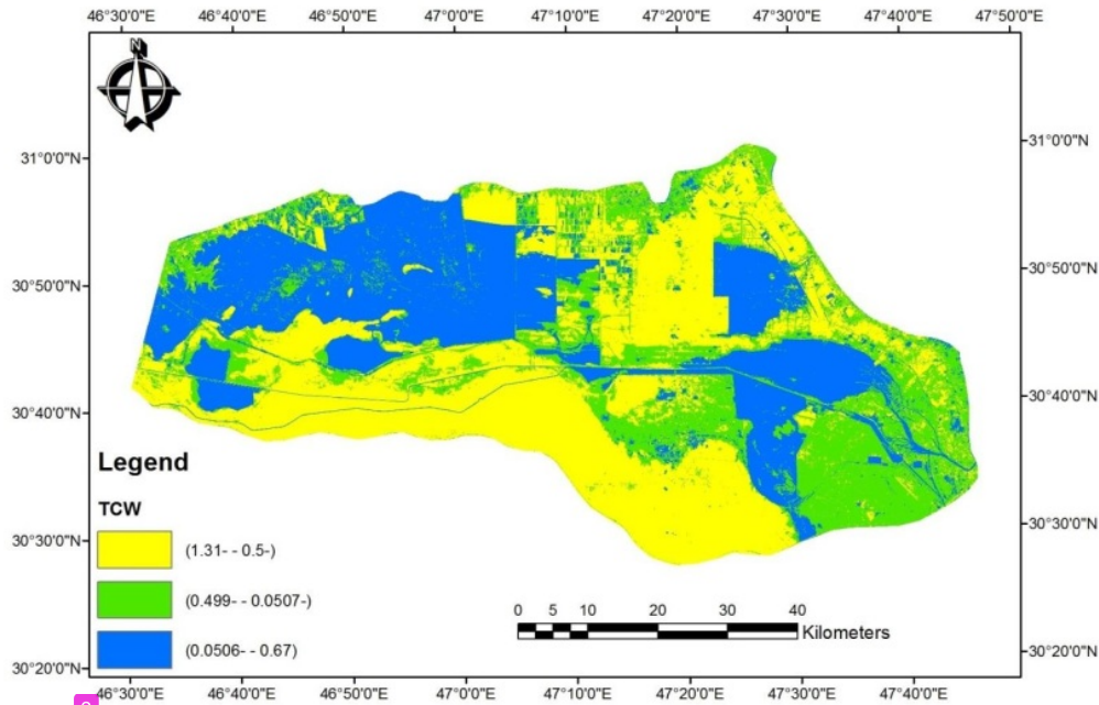
Figure (10) Spatial distribution of the TCW index for the year 2019
