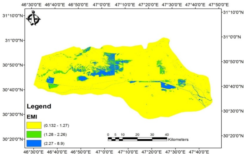
Figure (4) Spatial distribution of the EMI index for the year 2019
