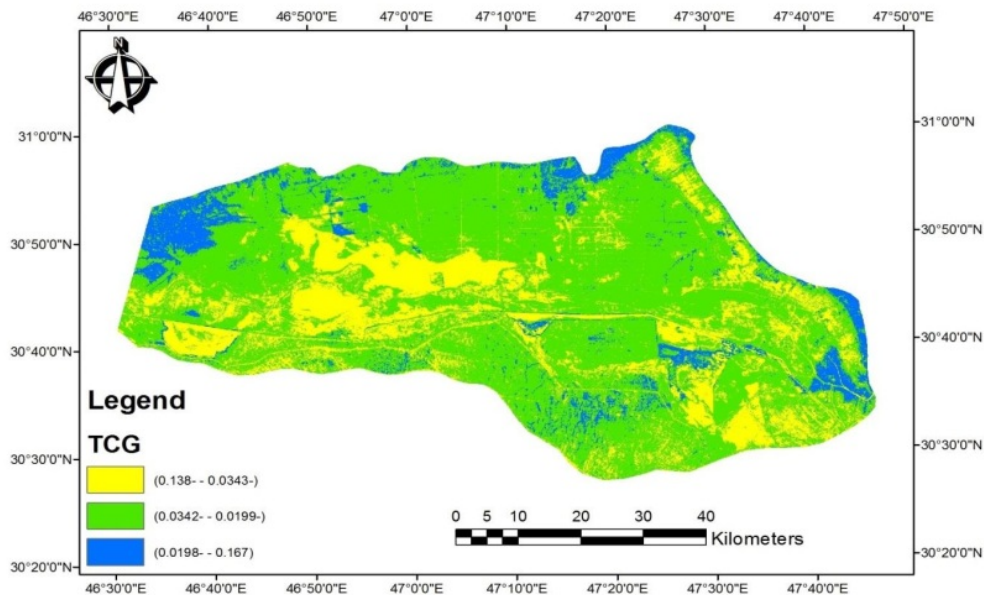
Figure (11) Spatial distribution of the TCG index for the year 2006
