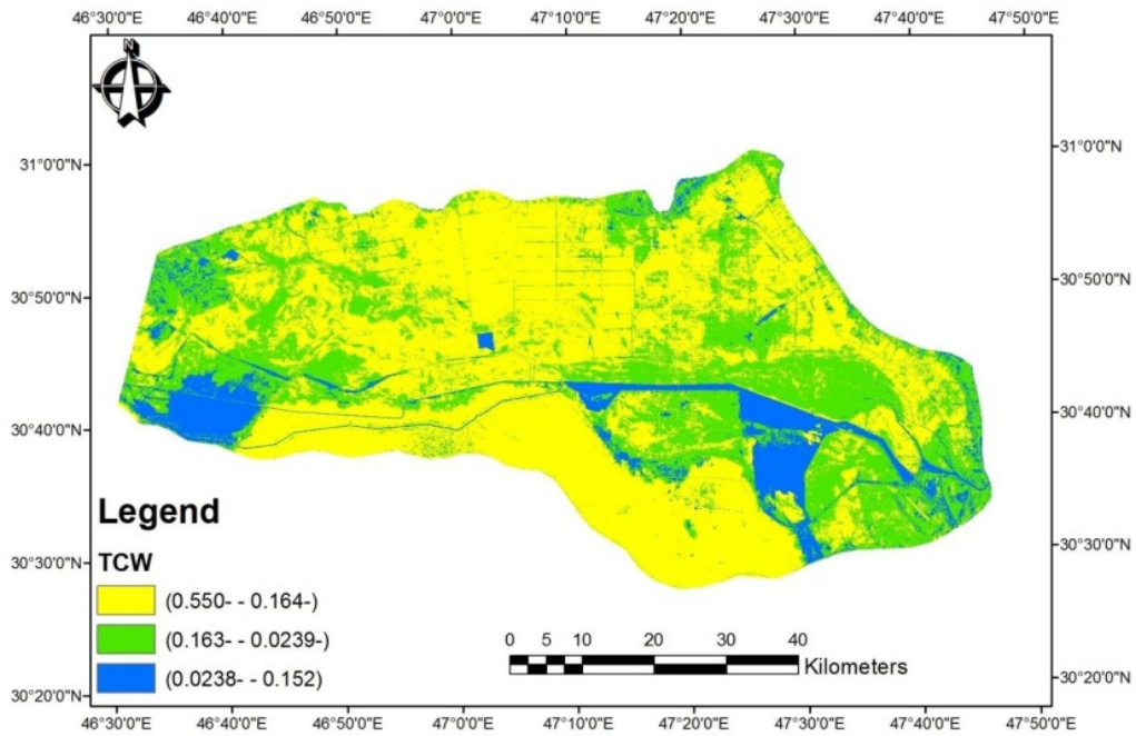
2 Figure (8) Spatial distribution of the TCW index for the year 2006
