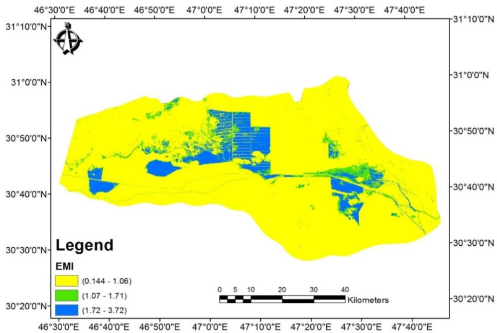
Figure (3) Spatial distribution of the EMI index for the year 2014
