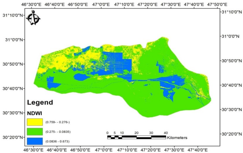
2 Figure (6) Spatial distribution of the NDWI index for the year 2014
