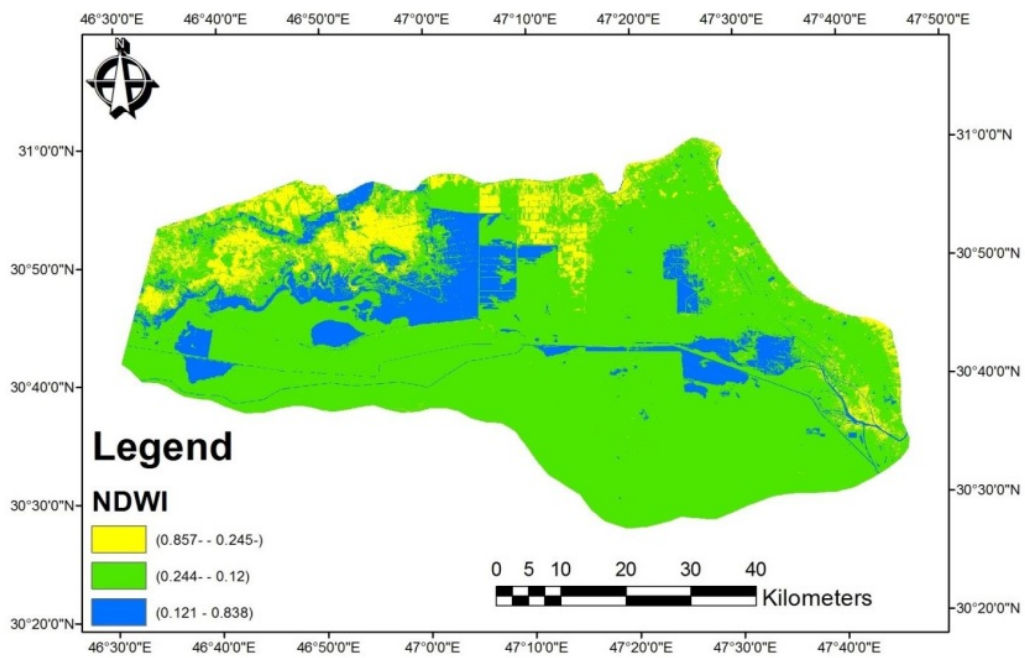
Figure (7) Spatial distribution of the NDWI index for the year 2019
