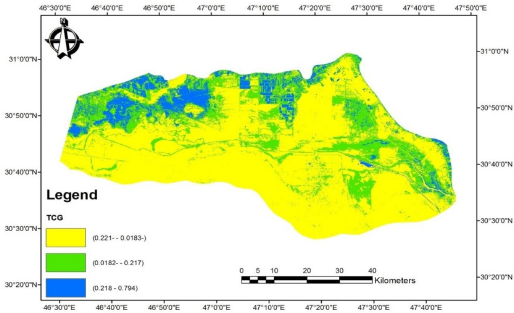
2 Figure (13) Spatial distribution of the TCG index for the year 2019
