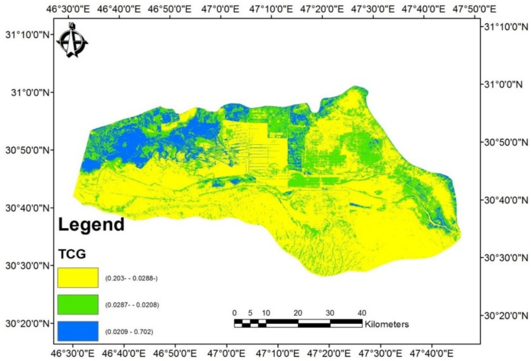
2 Figure (12) Spatial distribution of the TCG index for the year 2014
