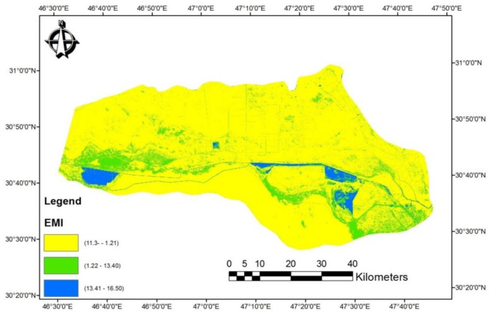
Figure (2) Spatial distribution of the EMI index for the year 2006
