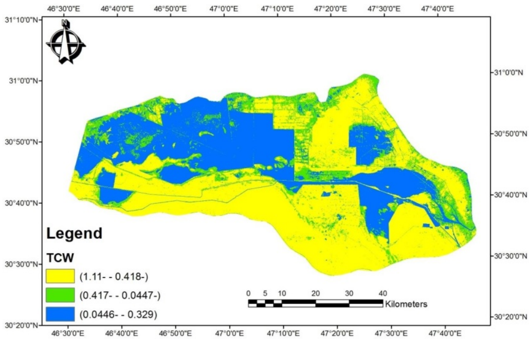
2 Figure (9) Spatial distribution of the TCW index for the year 2014
