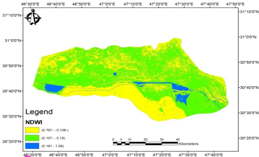
Figure (5) Spatial distribution of the NDWI index for the year 2006
