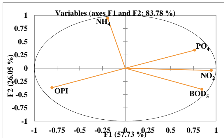
Fig 3. The PCA analysis between OPI and its correlated variables.
