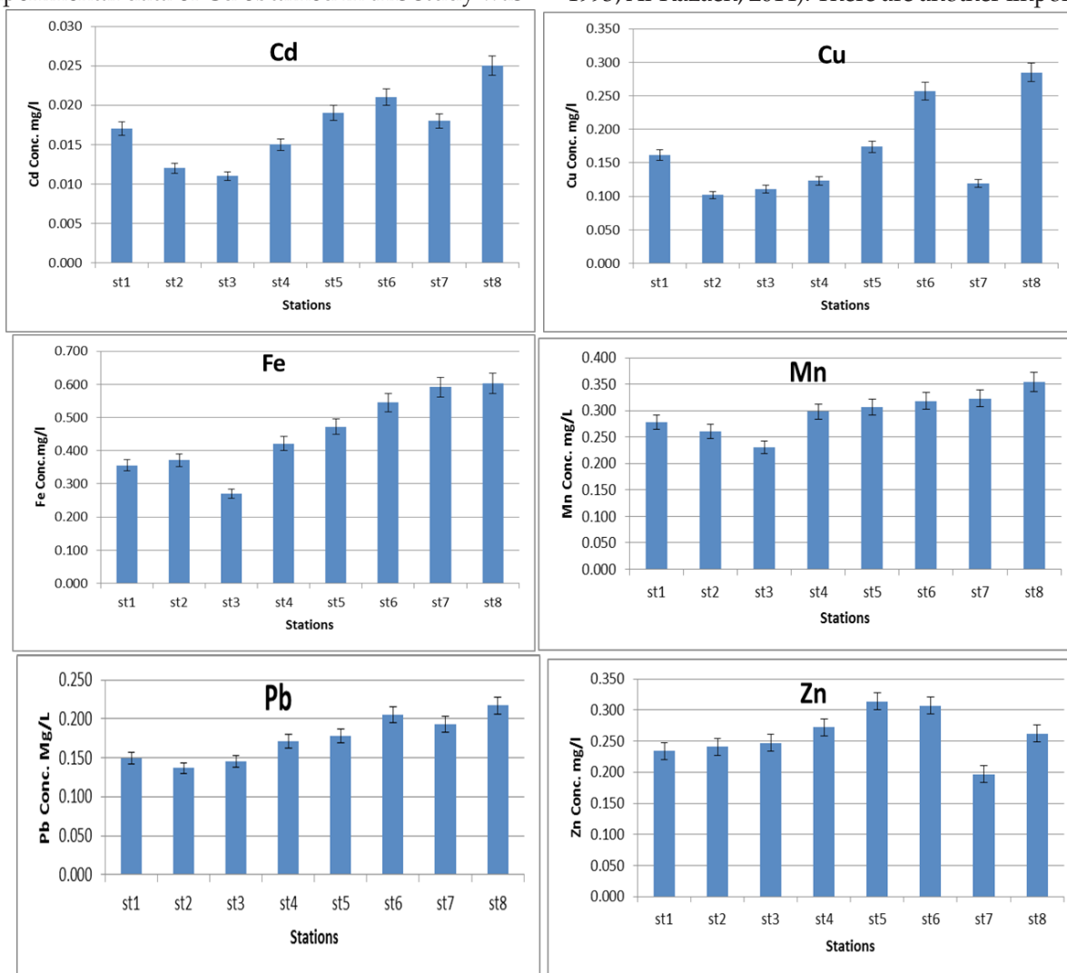
Fig. 2. The concentration of Cd, Cu, Fe, Mn, Pb and Zn (mg/L) in the stations of study area
