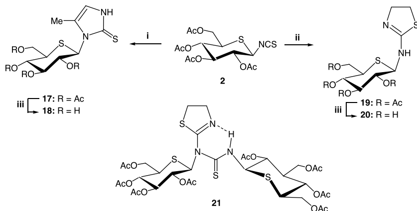
Scheme 2. Reagents and conditions: (i) \text{NH}_2\text{CH}_2\text{COMe.HCl}/\text{NaHCO}_3 , \text{Me}_2\text{CO} , 30 min, 23^\circ\text{C} ; (ii) \text{ClC}_2\text{H}_4\text{NH}_2.\text{HCl}/\text{H}_2\text{O}/\text{ether} , \text{M NaOH} , 15 h, 23^\circ\text{C} .
