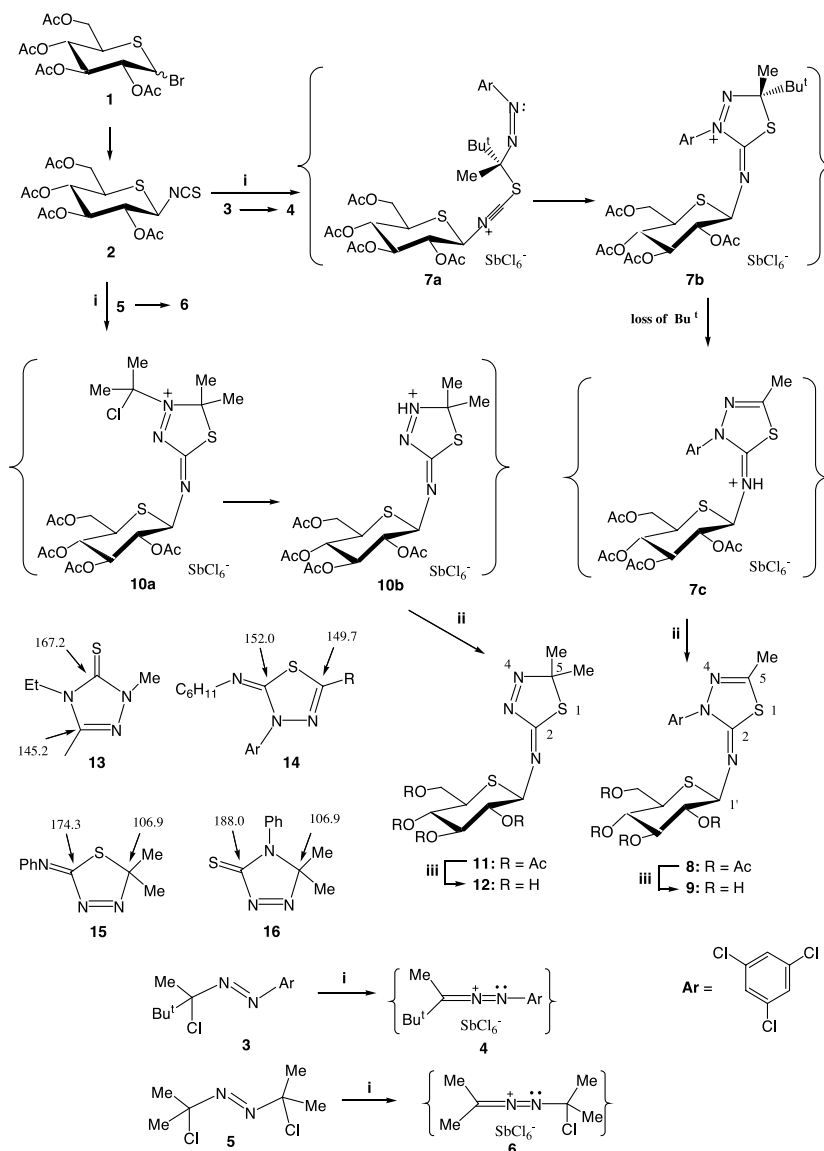
Scheme 1. Reagent and conditions: (i) \text{SbCl}_5 , \text{CH}_2\text{Cl}_2 , -60^{\circ}\text{C} to 23^{\circ}\text{C} , 7 h, \text{CH}_2\text{Cl}_2 , 23^{\circ}\text{C} ; (ii) aq. \text{NaHCO}_3 , 2 h, 23^{\circ}\text{C} , (iii) NaOMe, MeOH, 16 h, 23^{\circ}\text{C} .
