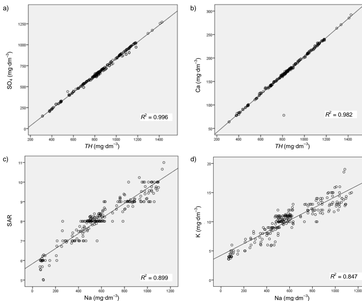
Fig. 3. The relationship between variables in the nine stations; a) TH vs. SO_4^{2-} , b) TH vs. Ca^{2+} , c) Na^+ vs. SAR, d) Na^+ vs. K^+ ; TH = total hardness, SAR = sodium adsorption ratio, R^2 = correlation coefficient; source: own study
