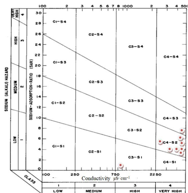
Fig. 4. Classification of water for irrigation; the mean values of the chemical data denoted as circles for water sampling sites; source: own study
