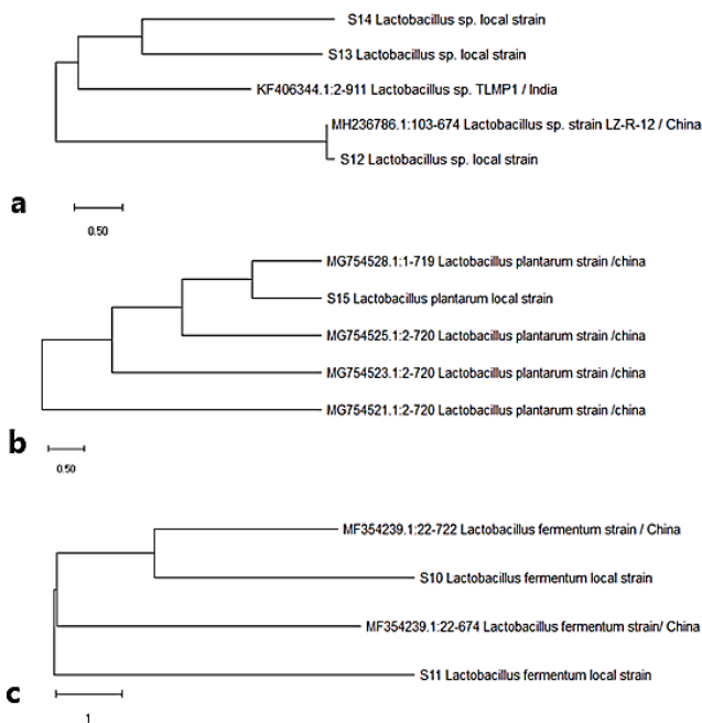
Figure 2: Phylogenetic tree analysis of a: Lactobacillus sp. b: Lactobacillus plantarum , c: Lactobacillus fermentum constructed based on 16S rRNA sequence analysis, showing the phylogenetic location of isolated strains from raw goat milk. The tree was constructed by the neighbor-joining statistical method, and GenBank ID of each strain used for contrast are given
