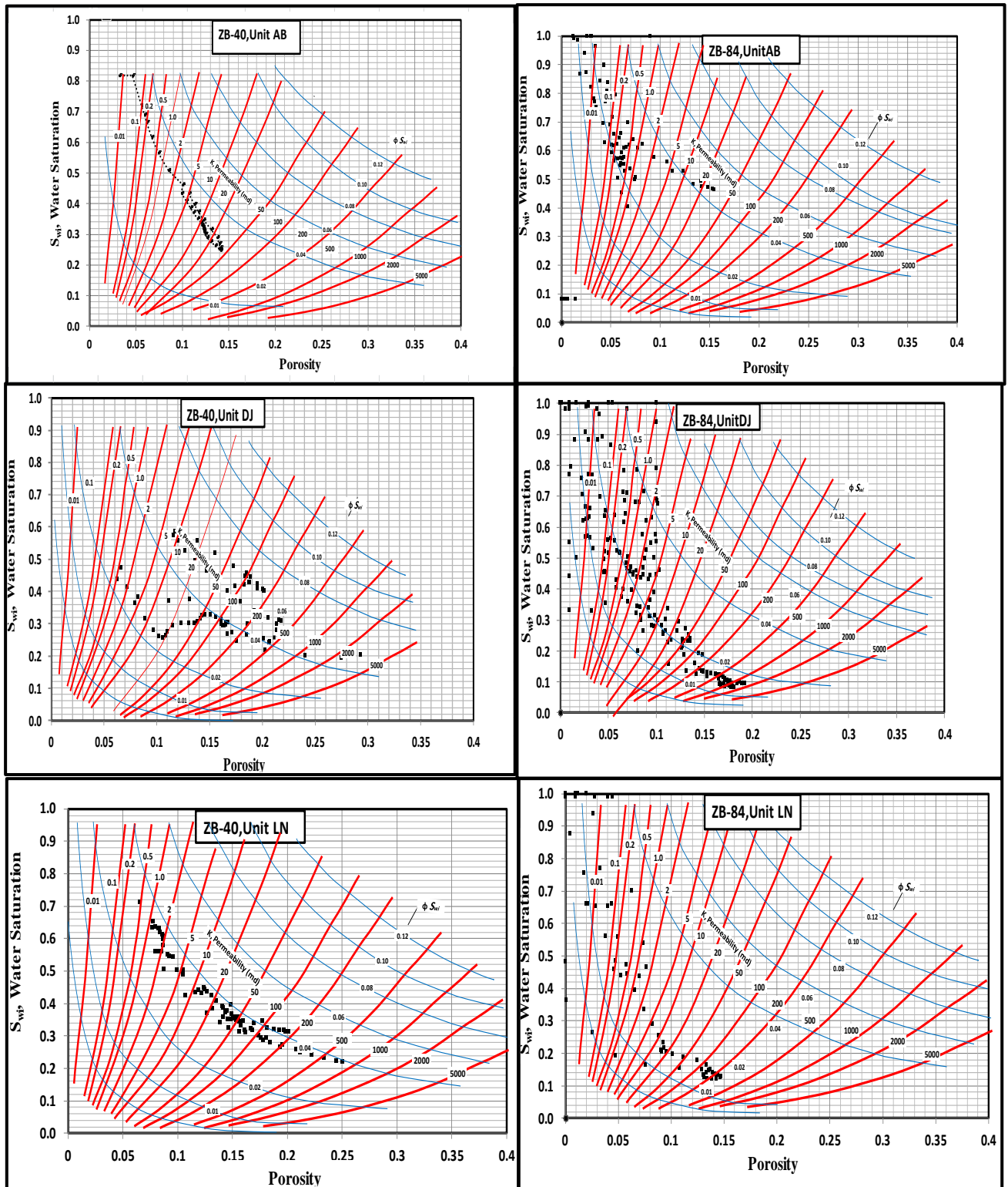
Fig. 13: Charts of ( \phi ) versus ( S_{wirr} ) for estimating permeability and determining (BWV) for the studied reservoir units within the wells (ZB-40,ZB-84) .
