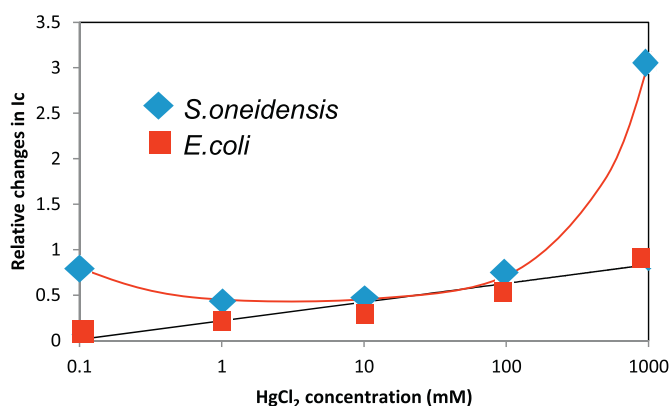
Fig. 9. The dependencies of relative changes of I_c of gold electrodes with immobilized S. oneidensis and E. coli bacteria vs. concentration of HgCl_2 .
