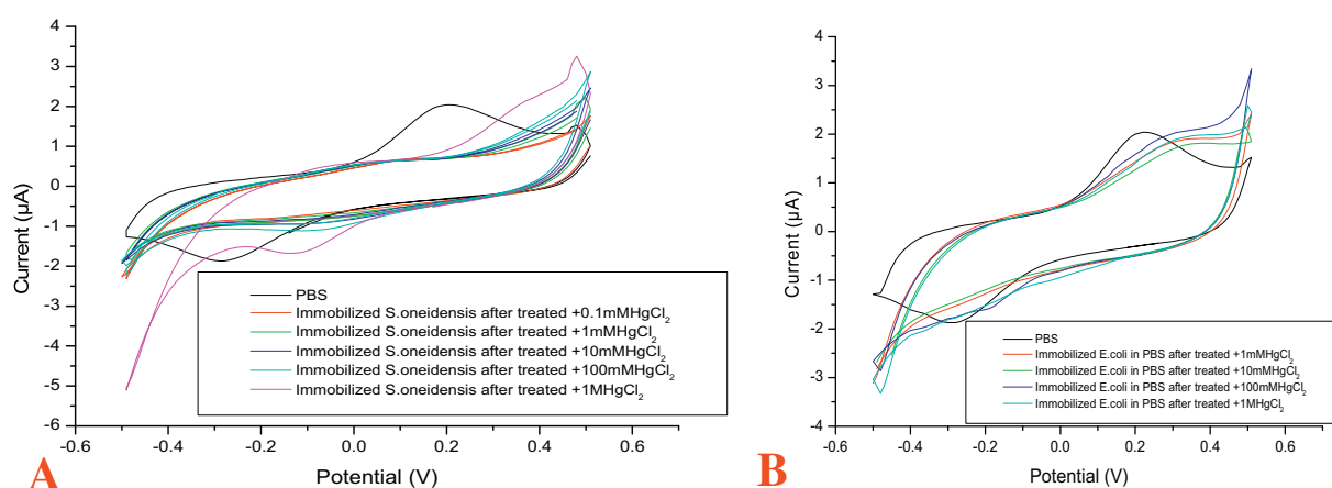
Fig. 8. CVs recorded on gold electrodes with immobilized S. oneidensis (A) and E. coli (B) bacteria in PBS, both before and after exposure to different concentrations of HgCl_2 .
