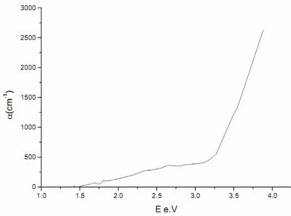
Fig. (4): Absorption coefficient ( \alpha ) as function of photon energy(E).
