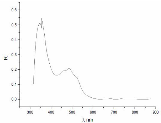
Fig. (7):Reflectance (R)as a function of wavelength( \lambda )
