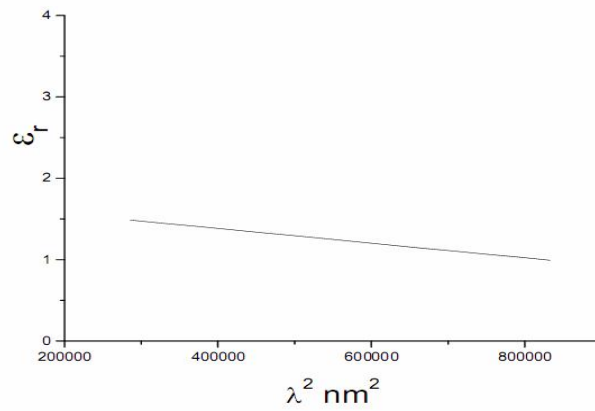
Fig. ( 12 ):Real part of dielectric constant ( \epsilon_r )as a function of square of wavelength ( \lambda^2 )
