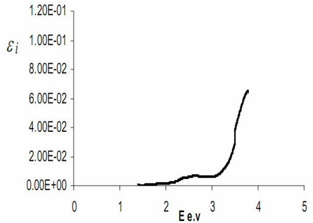
Fig. ( 11): Imaginary part of dielectric constant ( \epsilon_i ) as a function of photon energy(E)
