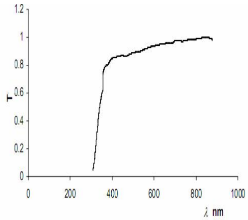
Fig.(3):The spectral transmission(T)As afunction of wavelength( \lambda )
