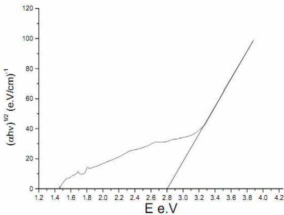
Fig. (6):Dependence of (\alpha h \nu)^{1/2} on the photon energy(E)
