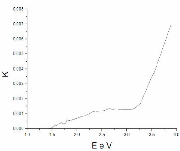
Fig. ( 8): Extinction coefficient (K)as function of photon energy(E)
