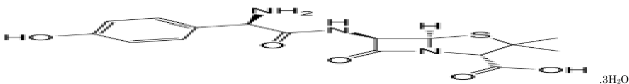
Fig. 1: Structural formula of amoxicillin trihydrate (AMX)
