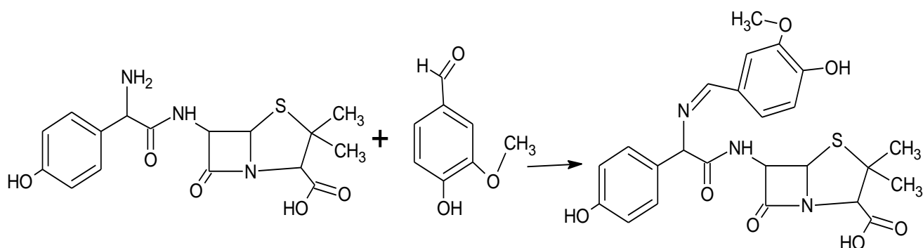
Scheme 1: Synthesis of amoxicillin Schiff base
